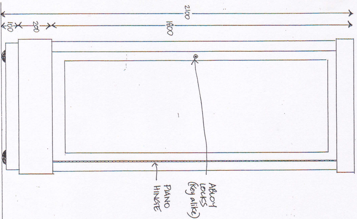
ELEVATION WITH DOOR:
