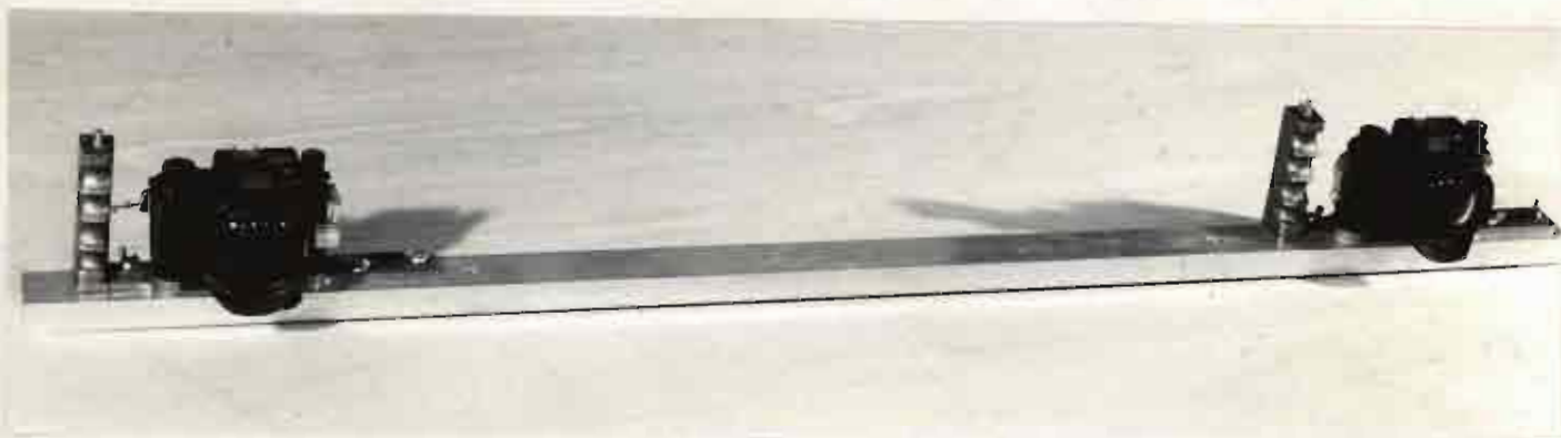
Fig. 8 Stereo bar with two Nikonos cameras with 15mm water corrected lenses. Camera separation 1 m.
